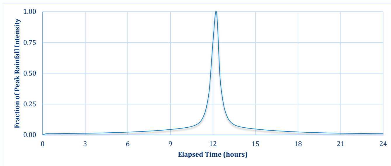
Figure 4-1: Design Storm Unit Hyetograph
