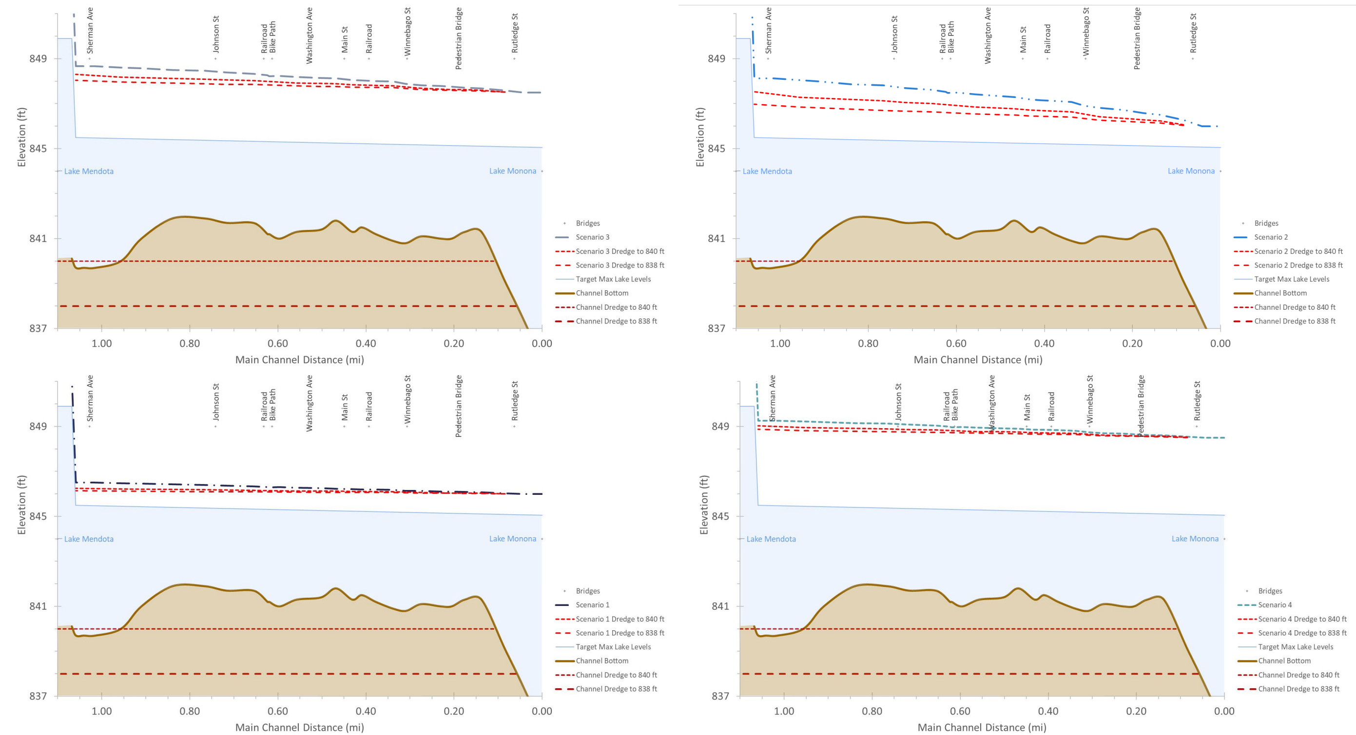
Figure 14-26: Yahara River – Dredging Results Scenarios 1-4
