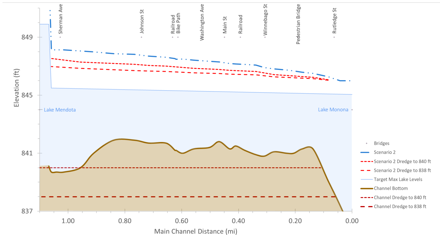
Figure 8-1: Scenario 2 – Model Dredging Results
